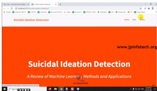
Fig.1. Home page.
